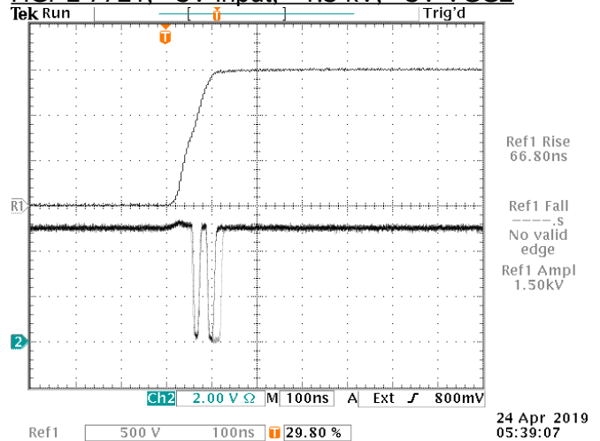
HCPL-7721, +5V input, +1.5 kV, +5V VCC2
