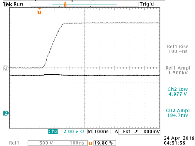
No DUT, +1.5 kV pulse, ~ 100 ns rise time
