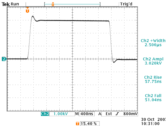
1 kHz, 2.5 us, +3000V into a 10 kΩ load. 500 V/div, 400 ns/div.
