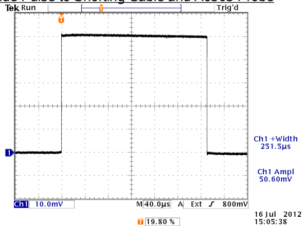
Wide Pulse to Shorting Cable and A6303 Probe
