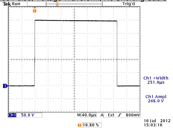
Wide Pulse, Voltage Waveform, No Shorting Cable
