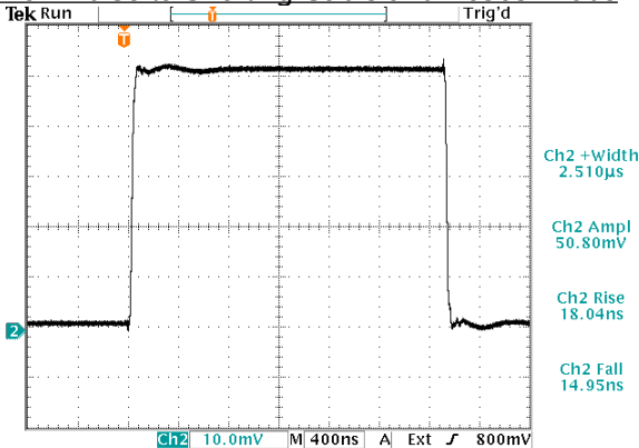
Narrow Pulse to Shorting Cable and A6303 Probe
