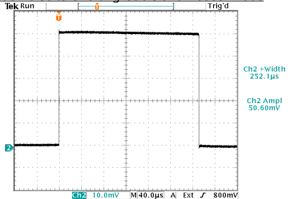
Wide Pulse to Shorting Cable and A6303 Probe
