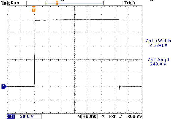
Narrow Pulse, Voltage Waveform, No Shorting Cable
