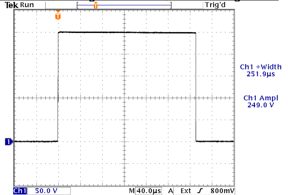
Wide Pulse, Voltage Waveform, No Shorting Cable
