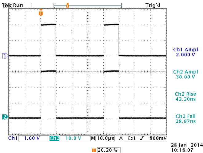
Top: +2V input, 1 V/div, 10 us/div. Bottom: output into 50Ω, +15 gain. 10 V/div, 10 us/div.
