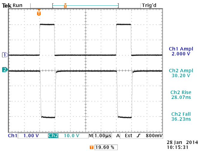
Top: +2V input, 1 V/div, 1 us/div. Bottom: output into 50Ω, -15 gain. 10 V/div, 1 us/div.
