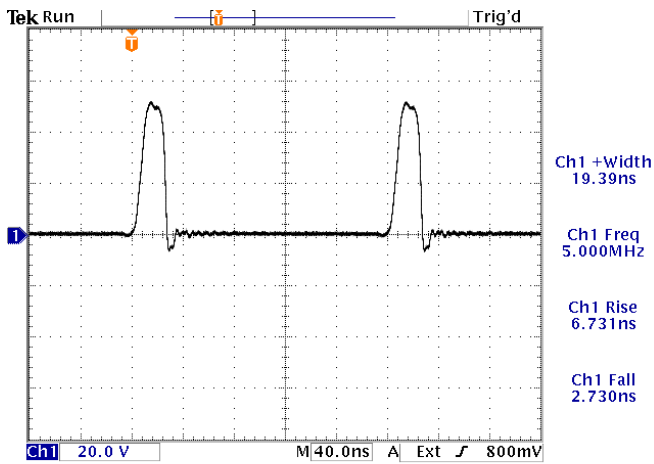
5 MHz, 20 ns, +50V, into 50 \Omega . 20V/div, 40 ns/div.
