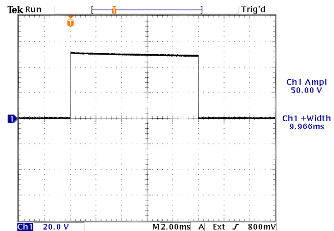
10 Hz, 10 ms, +50V, into 50 \Omega . 20V/div, 2 ms/div.
