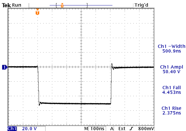
100 kHz, 500 ns, -50V, into 50 \Omega . 20V/div, 100 ns/div.
