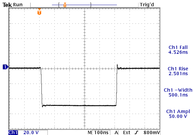
11 Sep 2020 19:58:05 20.00 % 100 kHz, 500 ns, -50V, into 50 \Omega . 20V/div, 100 ns/div.
