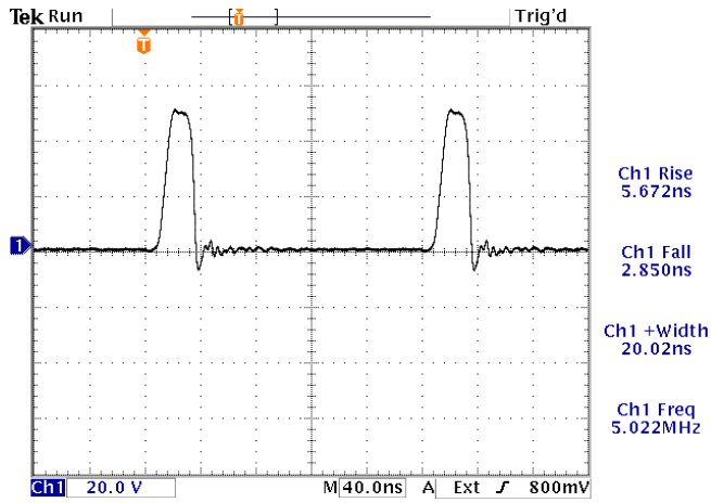
11 Sep 2020 19:57:06 19.80 % 5 MHz, 20 ns, +50V, into 50 \Omega . 20V/div, 40 ns/div.
