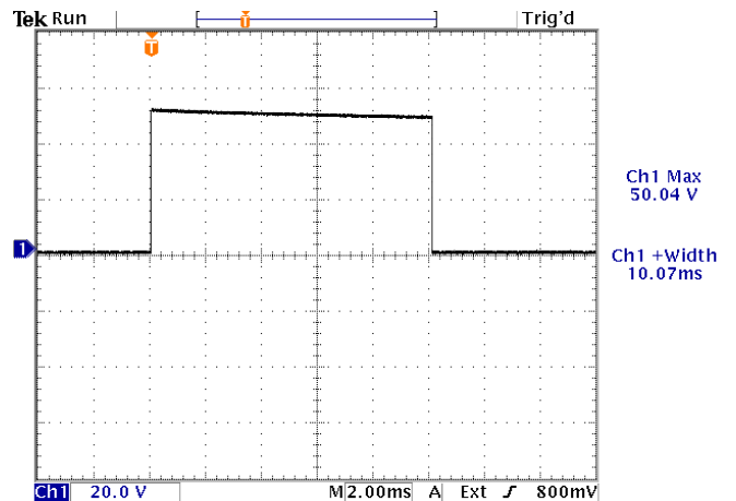
11 Sep 2020 19:59:28 20.40 % 10 Hz, 10 ms, +50V, into 50 \Omega . 20V/div, 2 ms/div.
