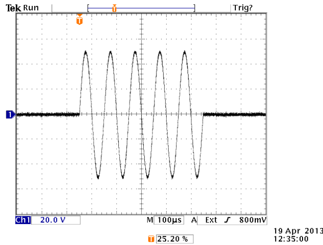
Sine burst mode, N = 5, 10 kHz. 20 V/div, 100 us/div.
