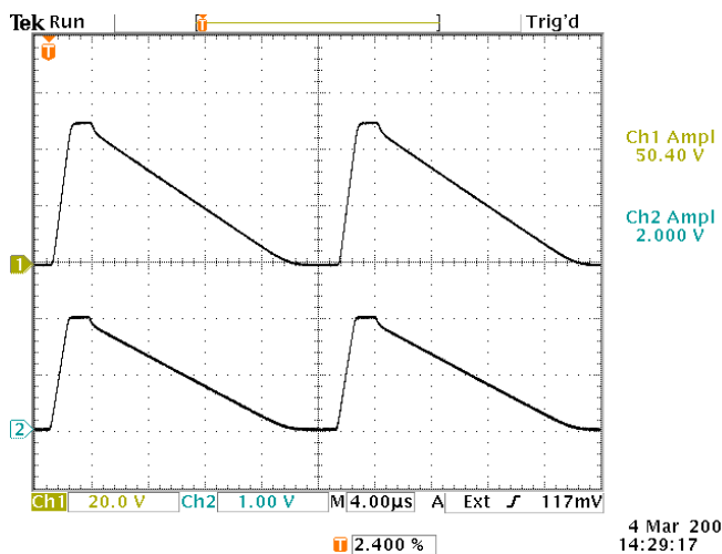
EXT mode, maximum gain. Top: +50V pulse out. 20 V/div, 4 us/div. Bottom: +2V pulse in. 1 V/div, 4 us/div.
