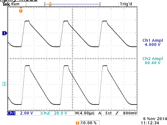
Top: ±2V arbitrary input. 2 V/div, 4 us/div. Bottom: amplified ±30V output. 20 V/div, 4 us/div.
