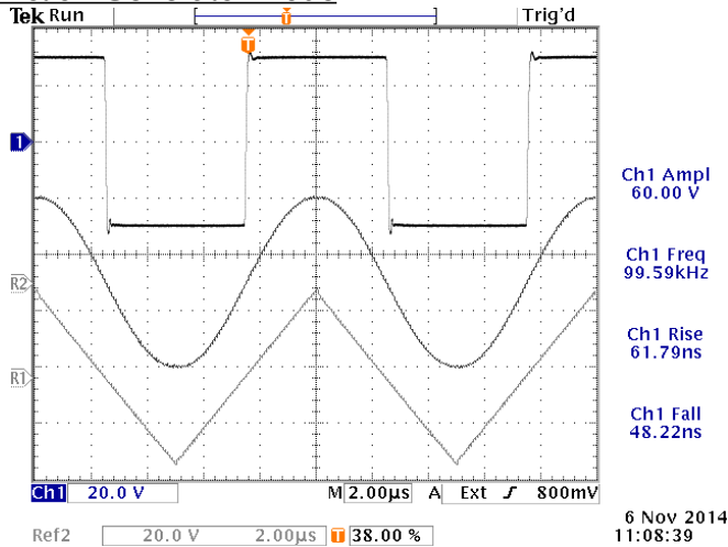
Square, Sine, and Triangle outputs into a 50Ω load. 100 kHz. 20 V/div, 2 us/div.
