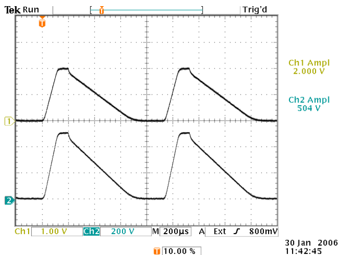
Amplify mode, maximum gain. Top: +2V pulse in. 1 V/div, 200 us/div. Bottom: +500V pulse out. 200 V/div, 200 us/div.
