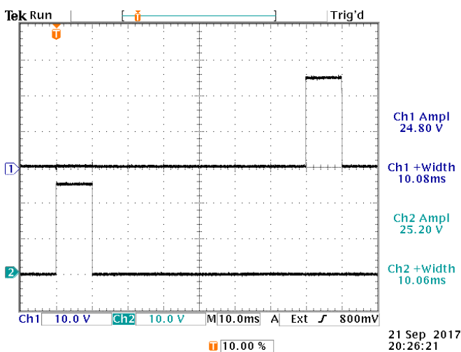
Top: OUT1, 10A into 2.5Ω, 10 ms PW, 70 ms delay Bottom: OUT2, 10A into 2.5Ω, 10 ms PW Both: 10 V/div, 10 ms/div, PRF = 1 Hz.
