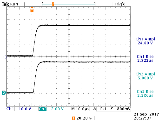
Top: OUT2, 10A into 2.5Ω load, 10 ms PW, 10 V/div. Bottom: MON2 into open circuit, 2V/div. Both: PRF = 1 Hz, 10 us/div.
