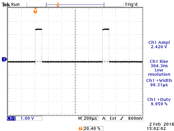
1000 Hz, 20 A, 100 us, into 0.12Ω. 1V/div, 200 us/div, using P5205 differential probe.
