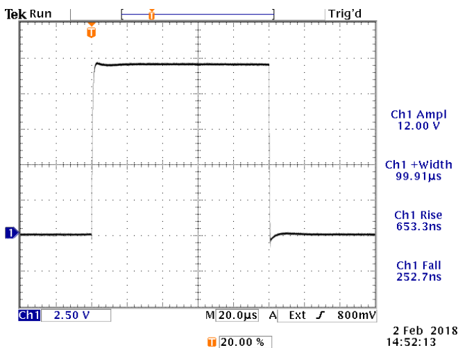
200 Hz, 100 A, 100 us, into 0.12Ω. 2.5V/div, 20 us/div, using P5205 differential probe.
