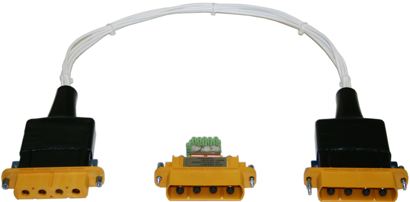
AV-HLZ2-100 output cable and mating AV-HLZAX Adapter / Test Load. (The green resistors soldered to the adapter in the photo are not included.)
