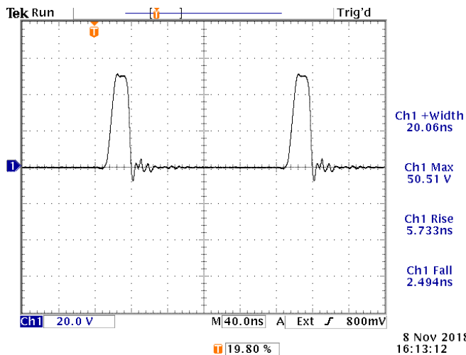
5 MHz, 20 ns, +50V, into 50 \Omega . 20V/div, 40 ns/div.
