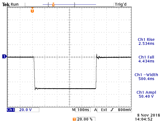
100 kHz, 500 ns, -50V, into 50Ω. 20V/div, 100 ns/div.
