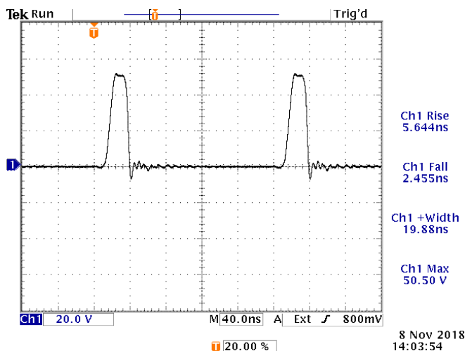
5 MHz, 20 ns, +50V, into 50Ω. 20V/div, 40 ns/div.
