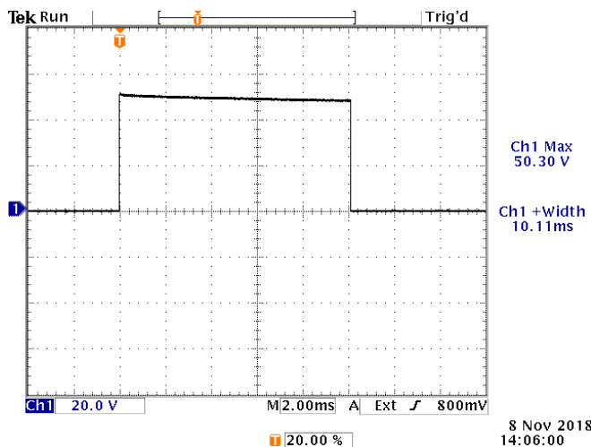
10 Hz, 10 ms, +50V, into 50Ω. 20V/div, 2 ms/div.
