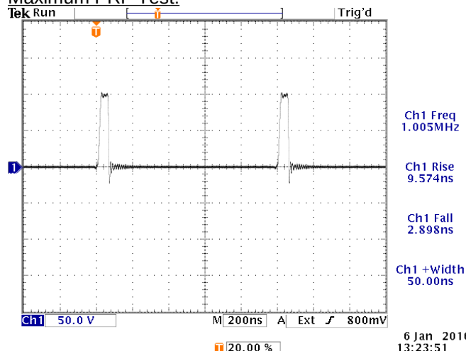
Maximum PRF Test:
