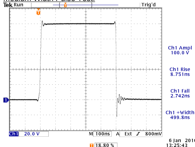
Medium Width Pulse Test:
