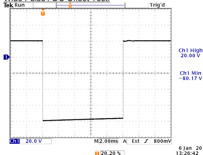
Wide Pulse / DC Offset Test:
