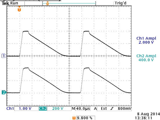
Top: +2V arbitrary input. 1 V/div, 40 us/div. Bottom: amplified 400V output. 200 V/div, 40 us/div.
