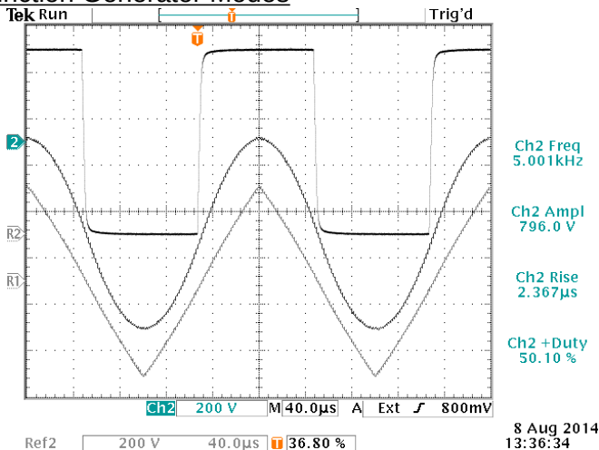
Square, Sine, and Triangle outputs into a 10 kΩ load. 5 kHz. 200 V/div, 40 us/div.
