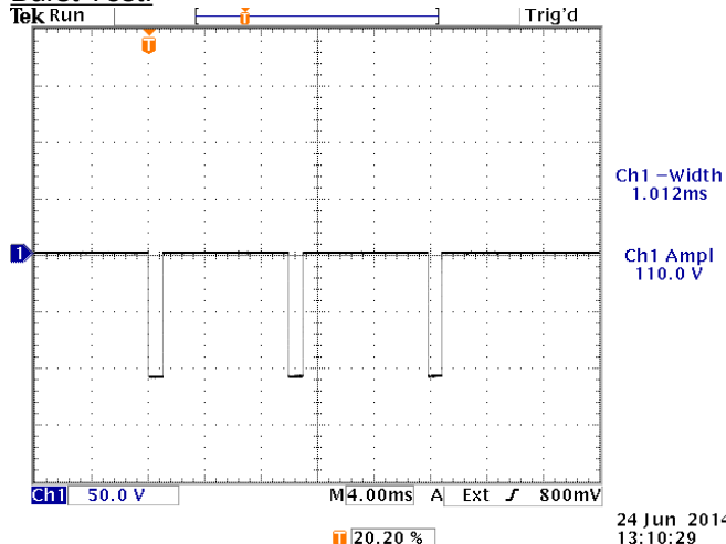
Output waveform (50V/div, 4 ms/div) for: PRF=10 Hz, PW=1 ms, AMPL=MIN, ZOUT=2Ω, BUR=9ms, N=3.
