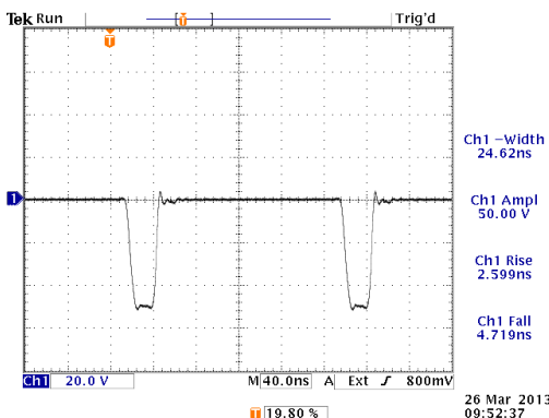
-50V, Z OUT =2Ω, 50Ω load, PW = 25 ns, 5 MHz
