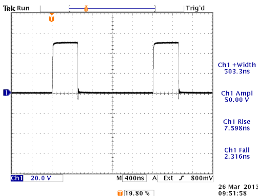
+50V, Z OUT =2Ω, 50Ω load, PW = 500 ns, 500 kHz
