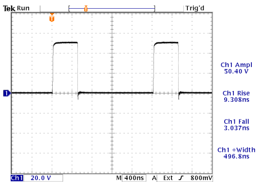
+50V, Z OUT =2Ω, 50Ω load, PW = 500 ns, 500 kHz
