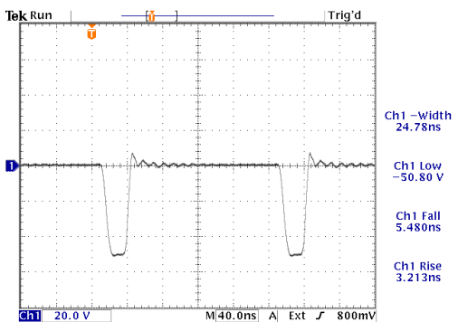
-50V, Z OUT =2Ω, 50Ω load, PW = 25 ns, 5 MHz
