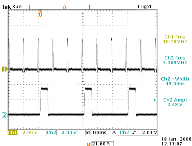
Top: TTL input, 10 MHz, 50Ω R IN . Bottom: TTL output, ÷3, 50 ns pulse width, 50Ω load. Both: 2V/div, 100 ns/div.
