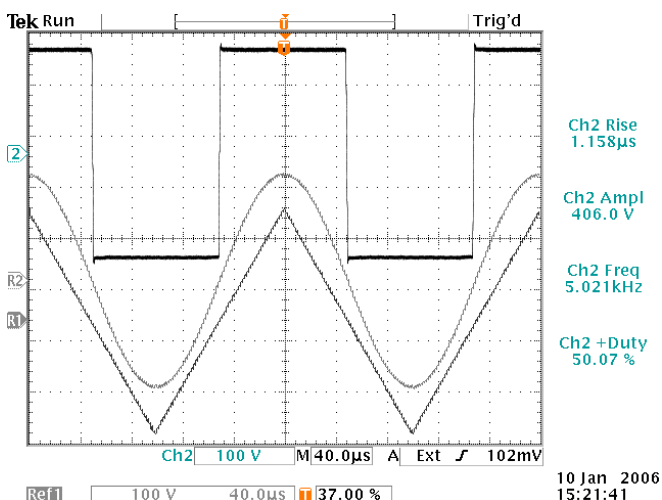
Square, Sine, and Triangle outputs into a 51 kΩ load. 5 kHz. 100 V/div, 40 µs/div.
