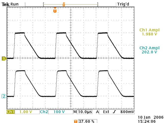
EXT mode, maximum gain. Top: +2V pulse in. 1V/div, 10 µs/div. Bottom: +200V pulse out. 100V/div, 10 µs/div.
