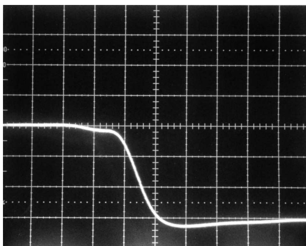
-3V output into 50 Ohms. 1 V/div, 1 ns/div.
