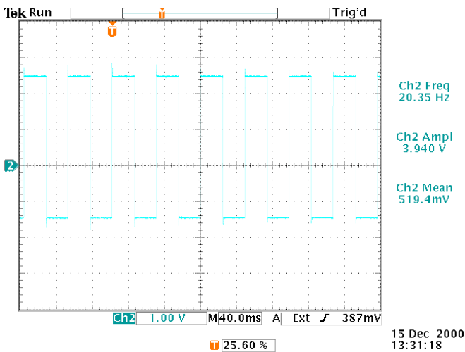
Top: OUT, \pm 2A (4A peak to peak) into a 1\Omega load 20 Hz, square wave output, offset of +0.5 A
