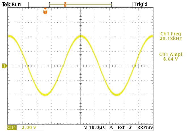
Top: OUT, \pm 2A (4A peak to peak) into a 2.0\Omega load 20 kHz, sine wave output, offset off
