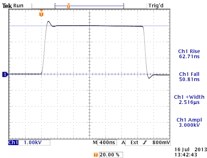
1 kHz, 2.5 us, +3000V into a 10 kΩ load. 1000 V/div, 400 ns/div.
