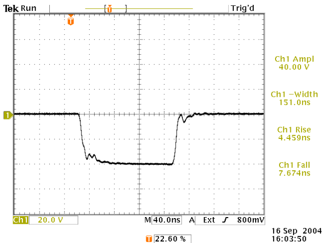
100 Hz, 150 ns, -40V into a 2Ω load. 20 V/div, 40 ns/div.
