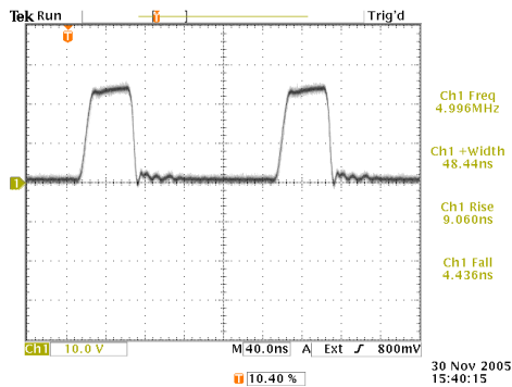
+50V, Z_{OUT}=50\Omega , 50 \Omega load, PW = 50 ns, 5 MHz
