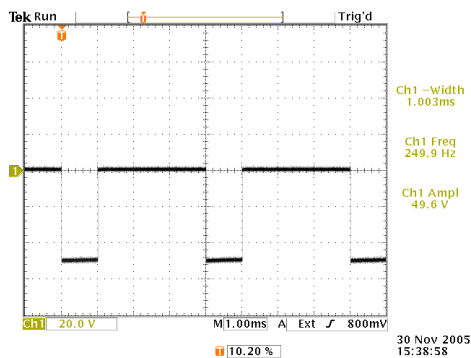
-50V, Z_{OUT}=2\Omega , 50 \Omega load, PW = 1 ms, 250 Hz
