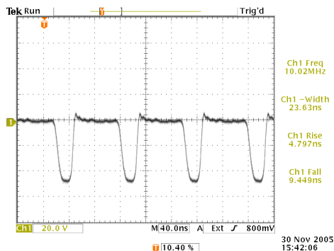
-50V, Z_{OUT}=2\Omega , 50 \Omega load, near minimum PW, 10 MHz
