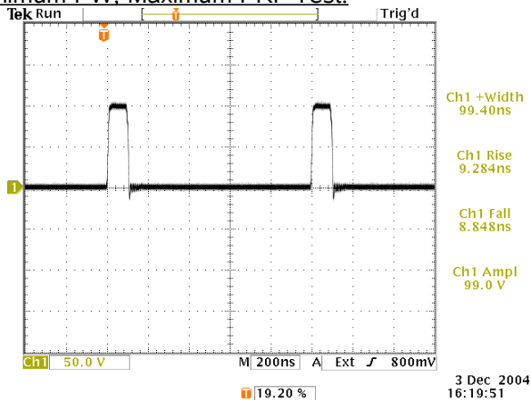
Output waveform (20V/div, 50 ns/div) for: PRF=1 MHz, PW=20ns, AMPL=+100V, ZOUT=2Ω
