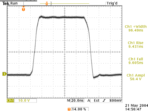
Output waveform (10V/div, 20 ns/div) for: PRF=1 MHz, PW=100ns, AMPL=+100V, ZOUT=50 \Omega
