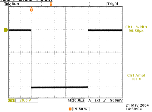
Output waveform (20V/div, 20 us/div) for: PRF=100 Hz, PW=100 us, AMPL=-100V, ZOUT=2 \Omega
