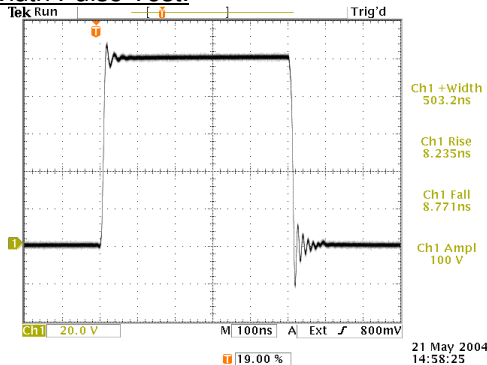
Output waveform (20V/div, 100 ns/div) for: PRF=100 kHz, PW=500ns, AMPL=+100V, ZOUT=2 \Omega
