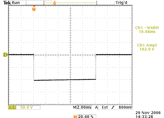
Output waveform (50V/div, 2 ms/div) for: PRF=5 Hz, PW=10 ms, AMPL=MIN, ZOUT=2Ω
