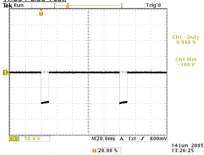
Output waveform (20V/div, 20 us/div) for: PRF=10 Hz, PW=10 ms, AMPL=-100V, ZOUT=2Ω
