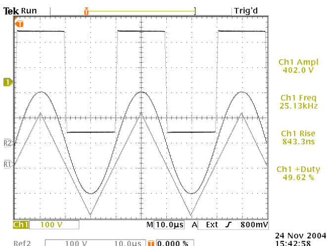
Square, Sine, and Triangle outputs into a 1.2 kΩ load. 25 kHz. 100 V/div, 10 us/div. References levels: 10%, 90%.
