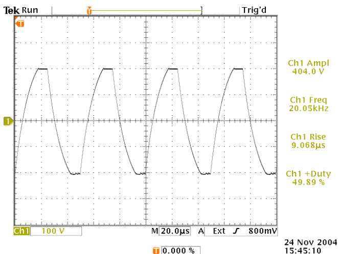
Square wave output into a load consisting of 1.2 kΩ and 10000 pF in parallel. 20 kHz, 20 us / div, 100 V/div. References levels: 20%, 80%.
