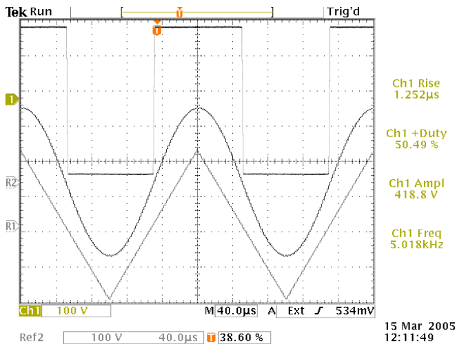
15 Mar 2005 12:11:49 Square, Sine, and Triangle outputs into a 51 kΩ load. 5 kHz. 100 V/div, 40 us/div.
