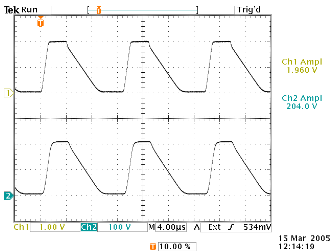
15 Mar 2005 12:14:19 EXT mode, maximum gain. Top: +2V pulse in. 1V/div, 4 us/div. Bottom: +200V pulse out. 100V/div, 4 us/div.
