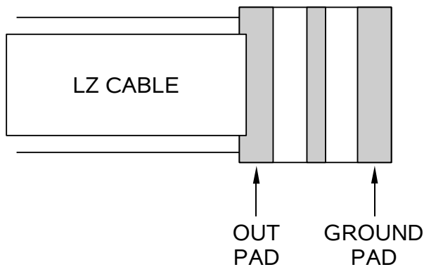
Layout of output end termination printed circuit board
