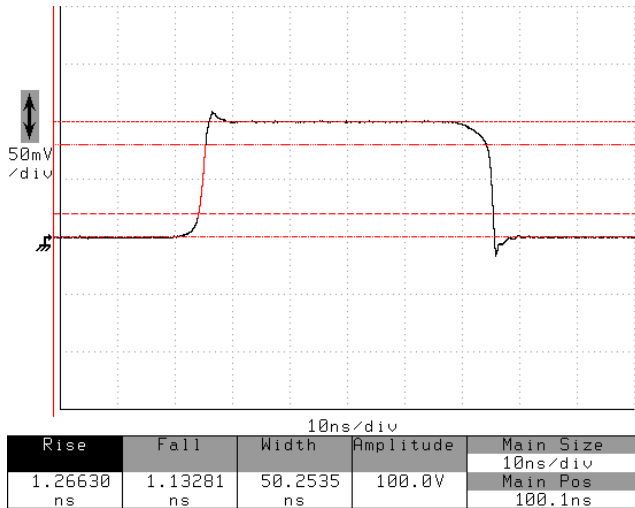
AVR-E3A-B-P, 10 kHz, 50 ns, +100V 50 V/div, 10 ns/div
