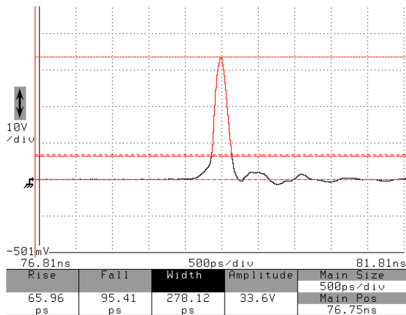
AVH-SB Series Output, 1 MHz, 10V/div, 500 ps/div.
