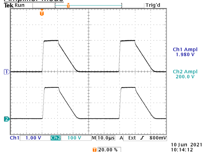
Top: +2V arbitrary signal in Bot: +200V amplified signal out, into 1.2 kΩ
