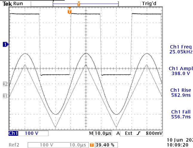
Square, Sine, and Triangle outputs into a 1.2 kΩ load at maximum amplitude. 25 kHz. 100 V/div, 10 us/div.
