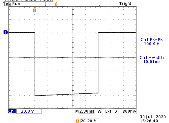
5 Hz, 10 ms, -100V. 20V/div, 2 ms/div.
