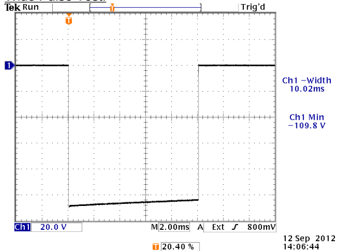
Output waveform (20V/div, 2 ms/div) for: PRF=5 Hz, PW=10 ms, AMPL=MIN, ZOUT=2Ω
