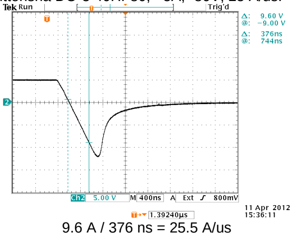
Ruttonsha DO-5 40HF80, +5A, -80V, 25 A/us.
