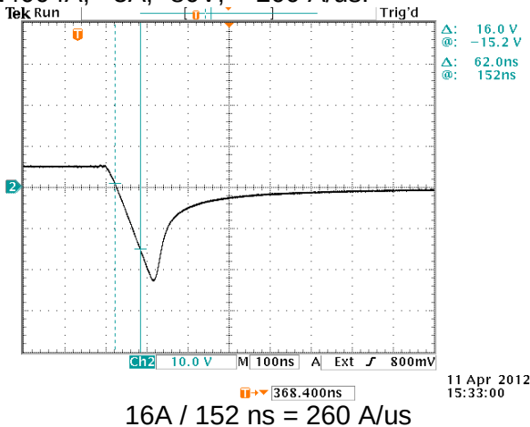
1N4004A, +5A, -80V, > 200 A/us.
