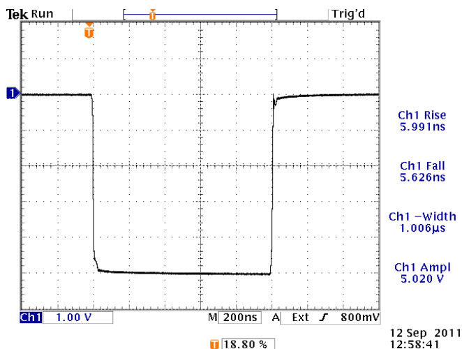
Output of Tektronix CT-2 current probe, measuring a -5A current pulse through a 1N5819 diode soldered to the output module. 1V & 1A/div, 200 ns/div.
