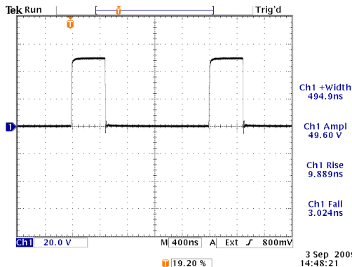
+50V, Z OUT =2Ω, 50Ω load, PW = 500 ns, 500 kHz
