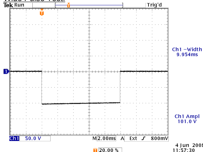
Output waveform (50V/div, 2 ms/div) for: PRF=5 Hz, PW=10 ms, AMPL=MIN, ZOUT=2Ω
