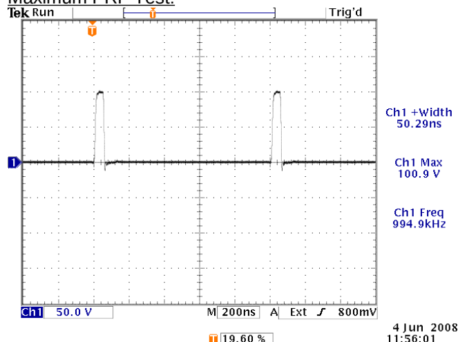
Output waveform (50V/div, 200 ns/div) for: PRF=1 MHz, PW=50 ns, AMPL=MAX, ZOUT=2Ω
