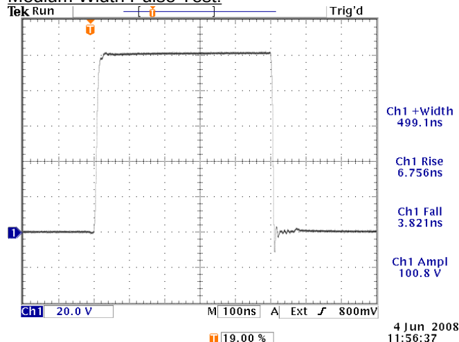
Output waveform (20V/div, 100 ns/div) for: PRF=100 kHz, PW=500ns, AMPL=MAX, ZOUT=2Ω
