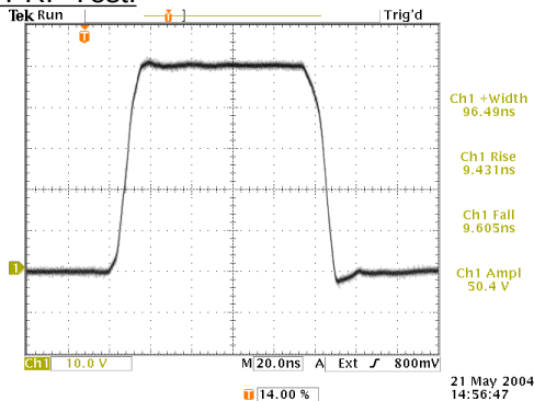
Output waveform (10V/div, 20 ns/div) for: PRF=1 MHz, PW=100ns, AMPL=+100V, ZOUT=50Ω
