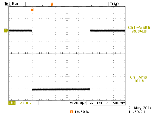
Output waveform (20V/div, 20 µs/div) for: PRF=100 Hz, PW=100 µs, AMPL=-100V, ZOUT=2Ω
