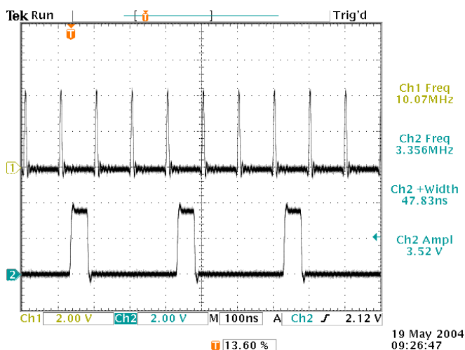
Top: TTL input, 10 MHz, 50Ω R IN . Bottom: TTL output, ÷3, 50 ns pulse width, 50Ω load. Both: 2V/div, 100 ns/div.
