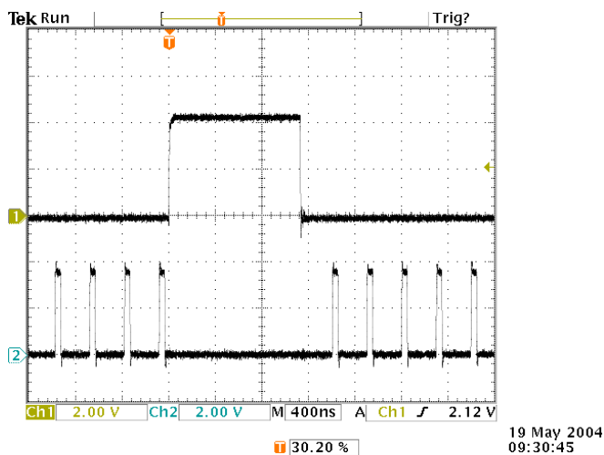
Top: RESET input. Bottom: TTL output, ÷3, f IN =10MHz. Both: 2V/div, 400 ns/div.
