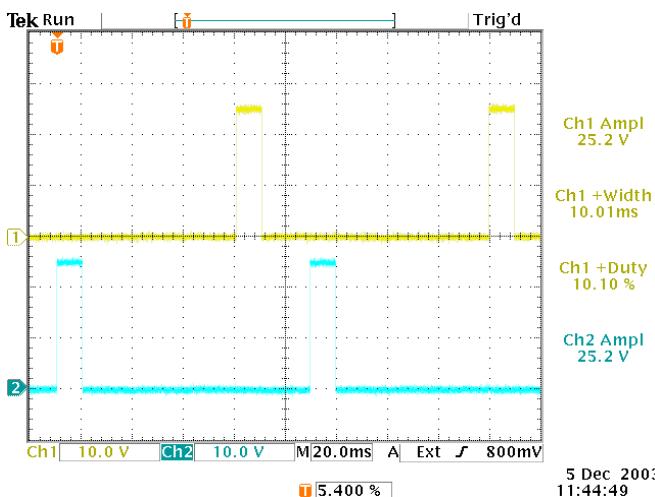
Top: OUT1, 5A into 5.0Ω load, 10 ms PW, 70 ms delay Bottom: OUT2, 5A into 5.0Ω load, 10 ms PW Both: 10 V/div, 20 ms/div, PRF = 10 Hz.
