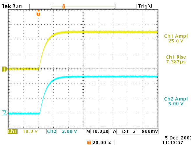
Top: OUT2, 5A into 5.0Ω load, 10 ms PW, 10 V/div. Bottom: M2 into 10 kΩ load, 2V/div. Both: PRF = 10 Hz, 10 us/div.
