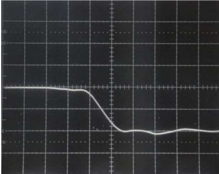
-2V output into 50 Ohms. 1 V/div, 1 ns/div.
