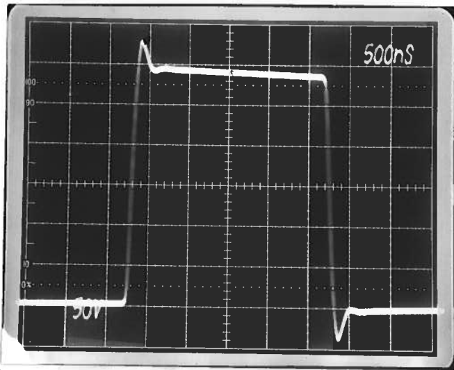
(A) P out , 500V/div, R L = 10K.
