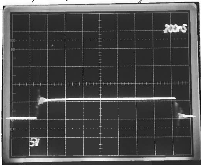
(B) AVO-6T OUT TO 1kΩ 50V/DIV 200NS/DIV
